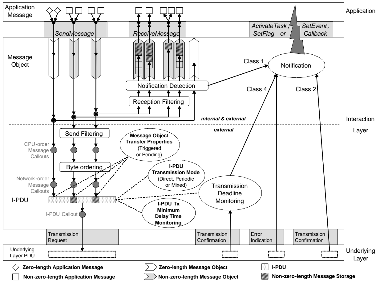
Figure 2-20: IL model for internal communication and external transmission
